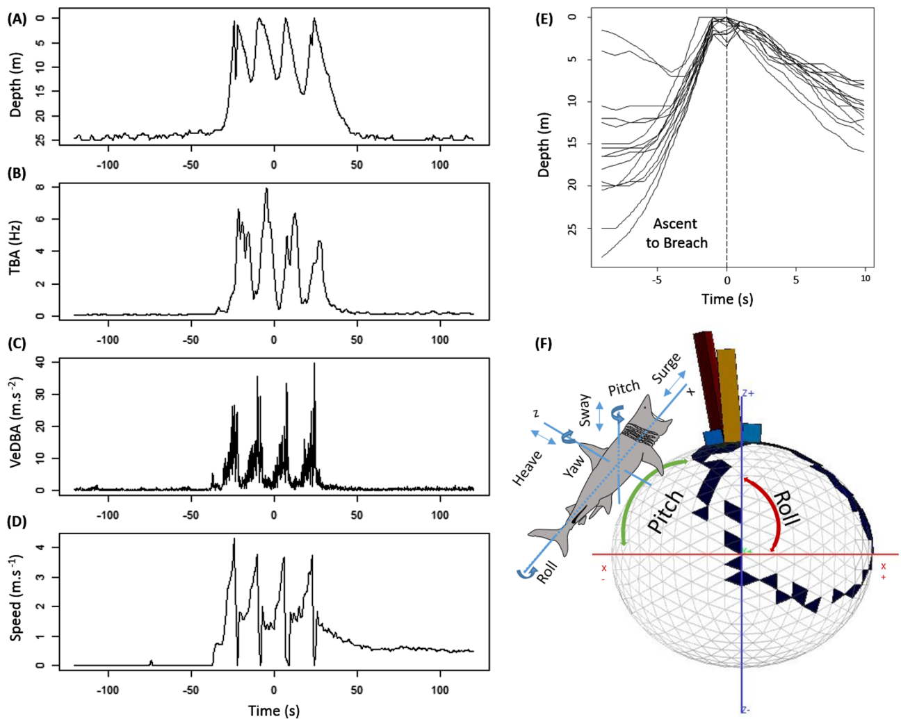
Figure 2. Characteristics of breaching. (A–D) A quadruple breach by a six-metre basking shark over 47 s showing changes in depth (A), tail beat amplitude (B), VeDBA (C) and speed (D) over the series of breaches. (E) Depth profiles of 16 single breaching events performed by a single shark, with time (in seconds) centred on the breach, overlaid on a common timescale showing repeatability of ascent angle and subsequent descent after breaching. (F) Dubai plot showing tri-axial acceleration data as a 3-dimensional histogram, with time spent by sharks in a particular posture on each facet of the sphere extruded as triangular bars, and colour scaling with the cumulative time in a given facet. Data show a right-handed breach of a single shark, where rapid rolling is indicated by short dark blue bars on the right face of the sphere.
